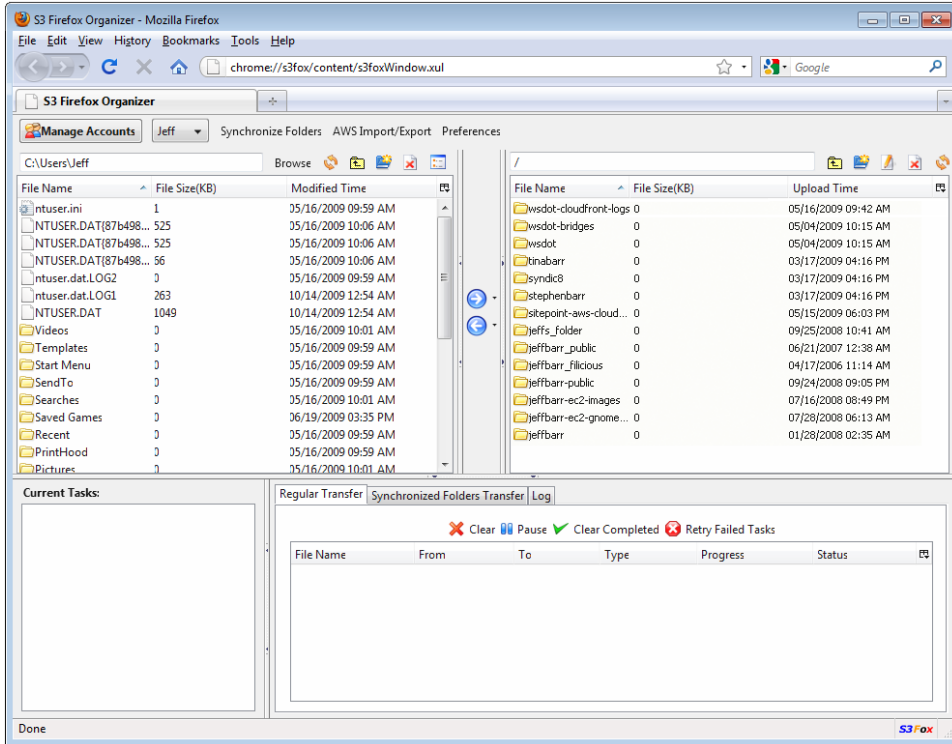
Figure 3.3. The S3Fox Organizer with its dual-paned approach
