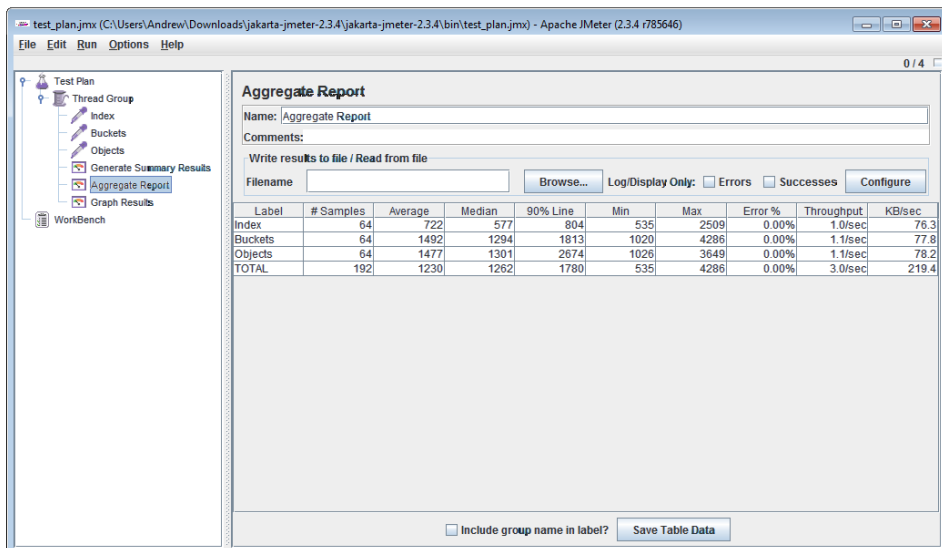
Figure 7.6. JMeter's Aggregate Report
