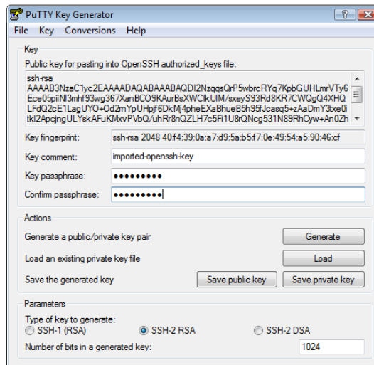
Figure 5.3. Adding a passphrase during key conversion
